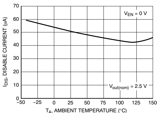
Figure 8. Disable Current vs. Ambient Temperature
