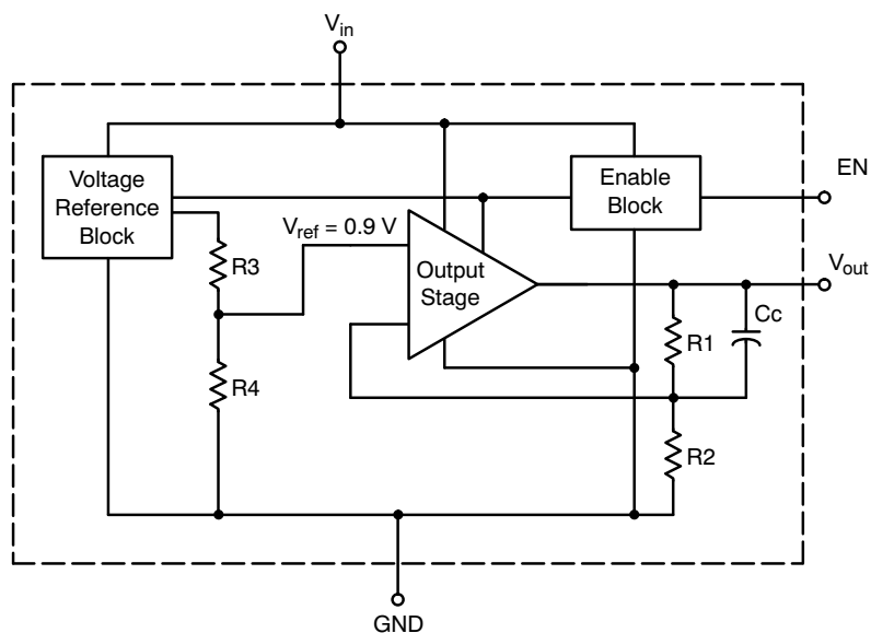
Figure 2. Block Diagram
