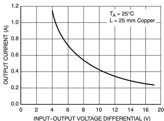
Figure 10. Output Current vs. Input-Output Voltage Differential
