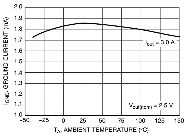
Figure 6. Ground Current vs. Ambient Temperature
