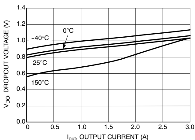
Figure 2. Dropout Voltage vs. Output Current
