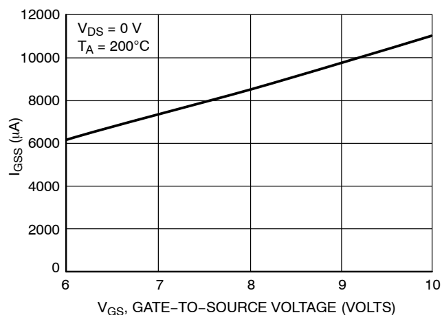
Figure 8. Input Current vs. Gate Voltage
