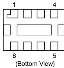
Figure 3. Pin Diagram
