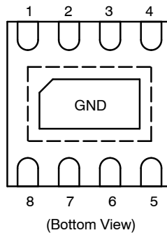
Figure 3. Pin Diagram
