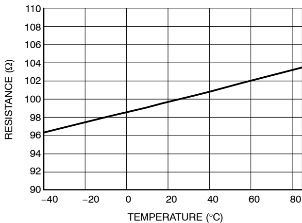
Figure 6. Typical Resistance over Temperature
