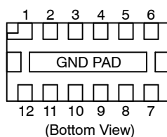
Figure 3. Pin Diagram
