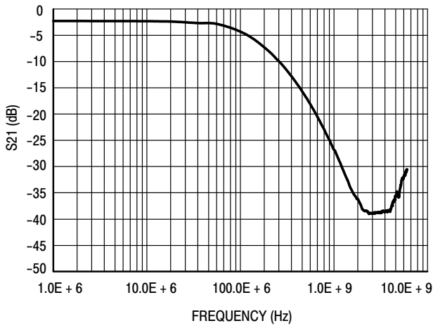
Figure 1. Typical Insertion Loss Characteristics (S21 Measurement)
