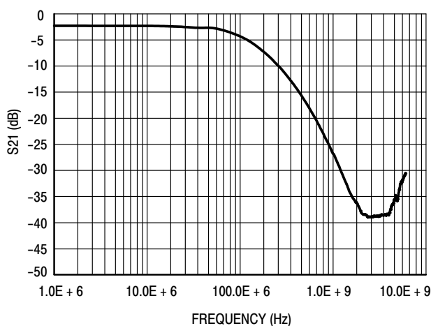
Figure 2. Typical Insertion Loss Characteristics (S21 Measurement)
