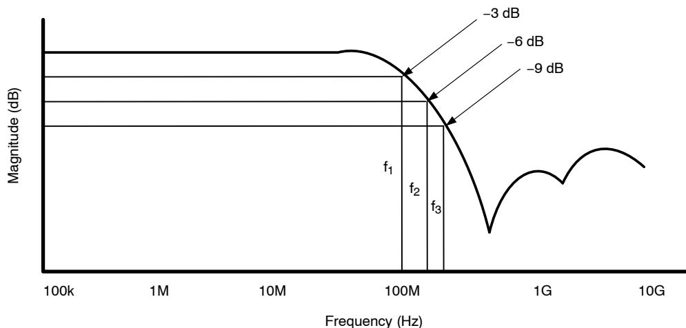
Figure 5. Filter Bandwidth
