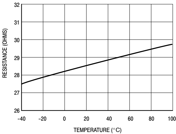
Figure 3. Typical Resistance Over Temperature
