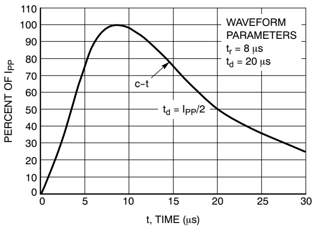
Figure 1. Pulse Waveform
