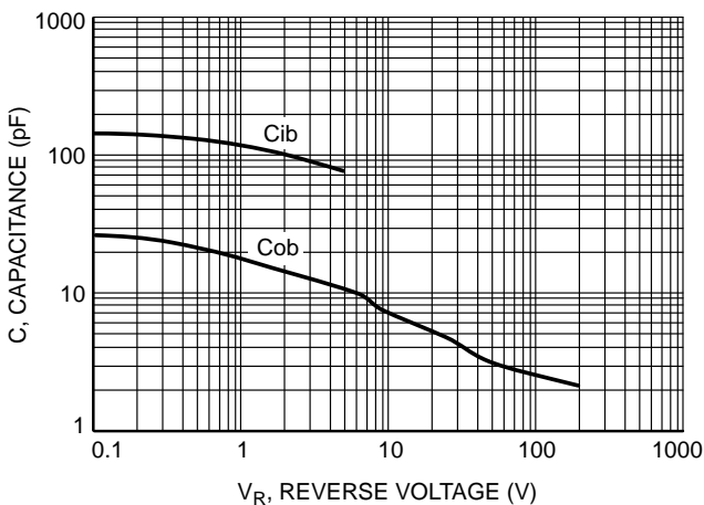
Figure 5. Capacitances
