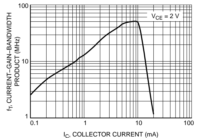
Figure 6. Current-Gain-Bandwidth Product
