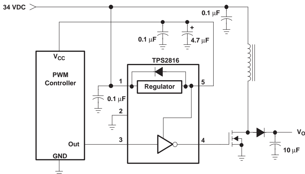
Figure 22. Boost Application
