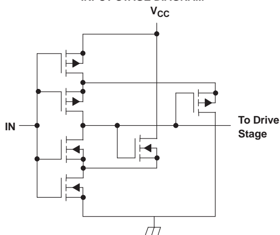
INPUT STAGE DIAGRAM
