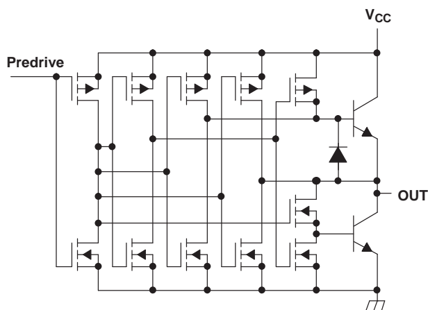
OUTPUT STAGE DIAGRAM
