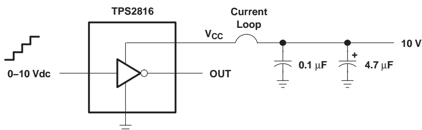
Figure 3. Shoot-Through Current Test Setup
