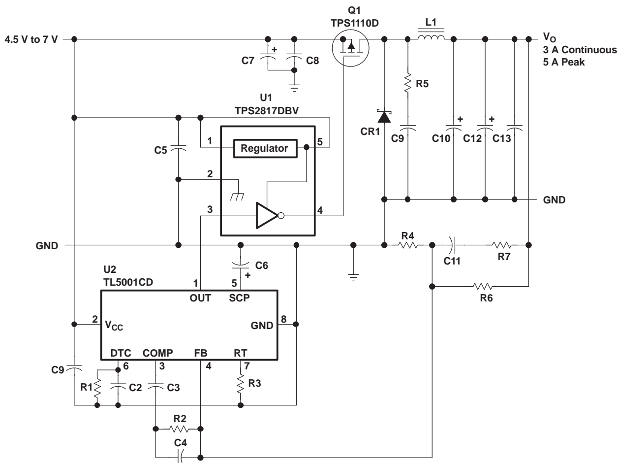
Figure 23. Step-Down Application
