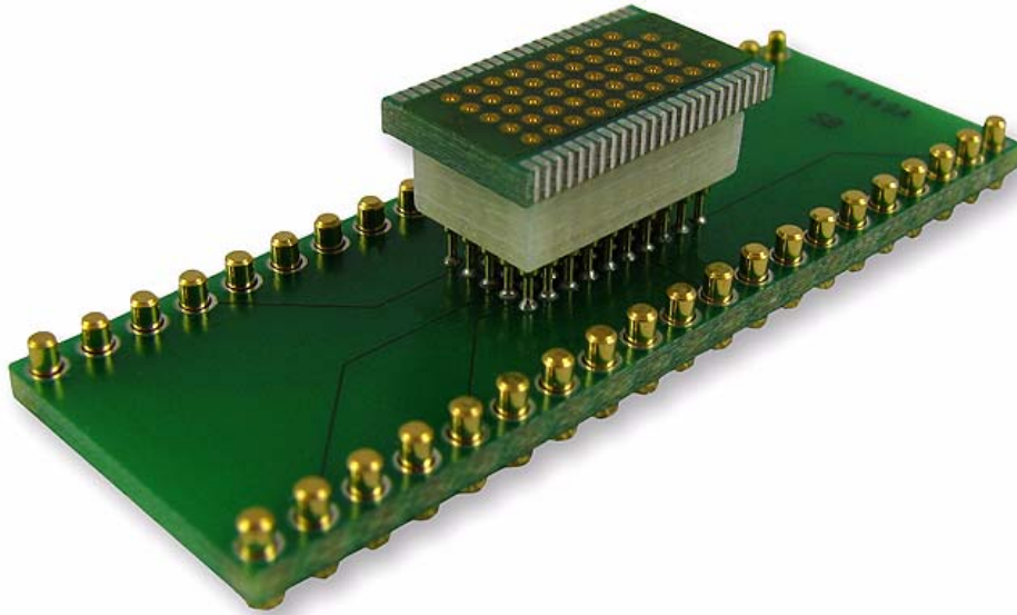
Figure 7. 40-PDIP to 48-SSOP Package Converter
