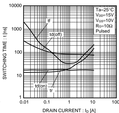
Fig.9 Switching Characteristics
