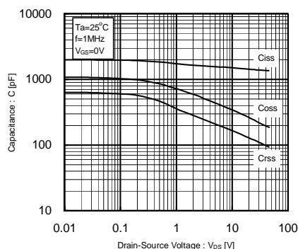
Fig.7 Typical capacitance vs. Source-Drain Voltage
