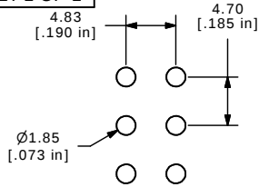
PC MOUNTING
