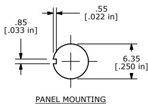
PANEL MOUNTING
