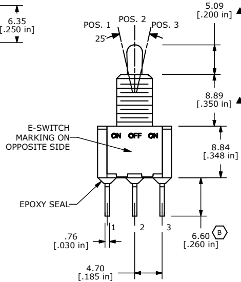
PANEL MOUNTING
