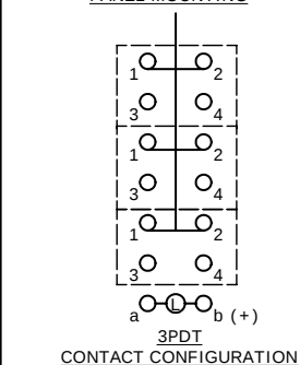
3PDT CONTACT CONFIGURATION
