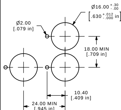
PANEL MOUNTING
