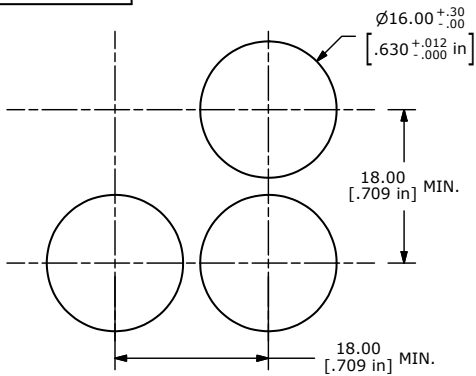
RECOMMENDED PANEL MOUNTING
