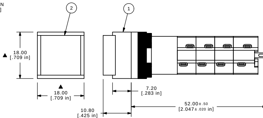
PANEL MOUNTING
