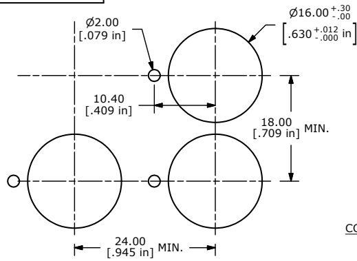
RECOMMENDED PANEL MOUNTING
