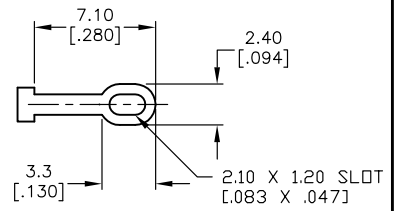
TERMINATION DETAIL SCALE 2X
