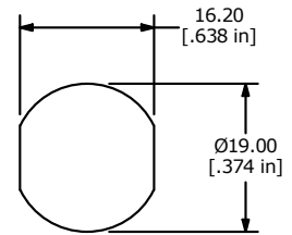
RECOMENDED PANEL CUTOUT
