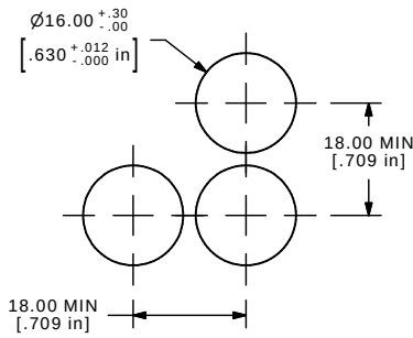
RECOMMENDED PANEL MOUNTING
