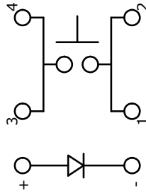
CIRCUIT: SPST
