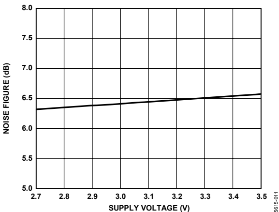
Figure 11. Noise Figure vs. Supply Voltage
