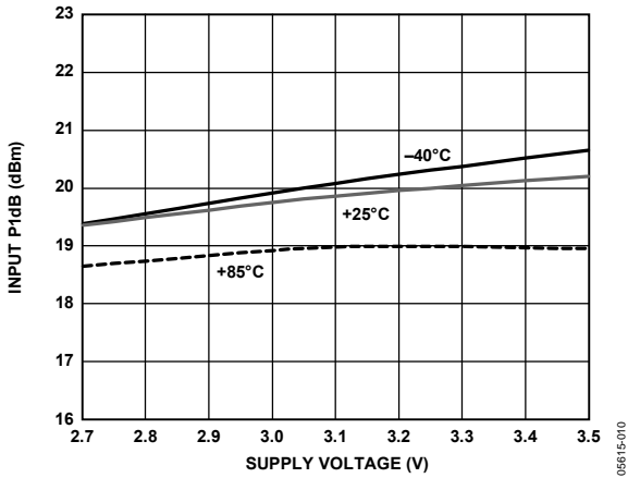
Figure 10. Input P1dB vs. Supply Voltage
