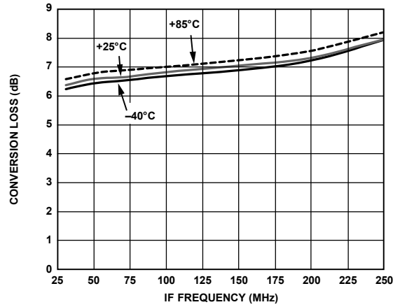
Figure 18. Conversion Loss vs. IF Frequency
