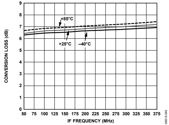
Figure 45. Conversion Loss vs. IF Frequency
