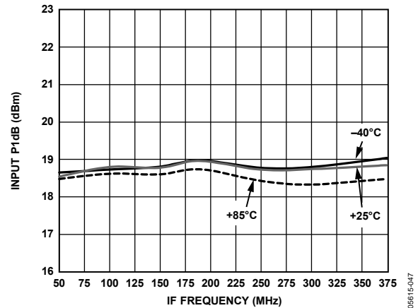
Figure 47. Input P1dB vs. IF Frequency
