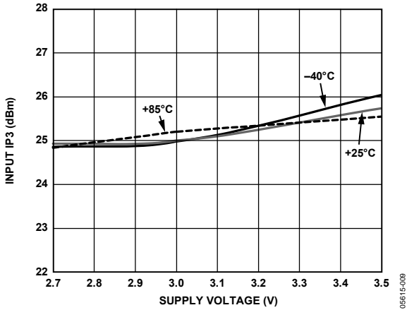
Figure 9. Input IP3 vs. Supply Voltage
