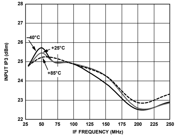
Figure 19. Input IP3 vs. IF Frequency
