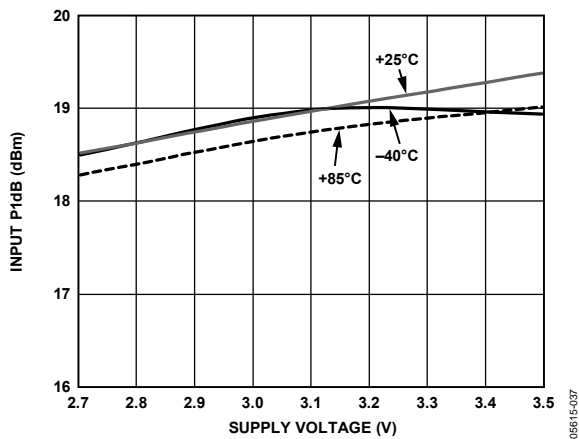
Figure 37. Input P1dB vs. Supply Voltage
