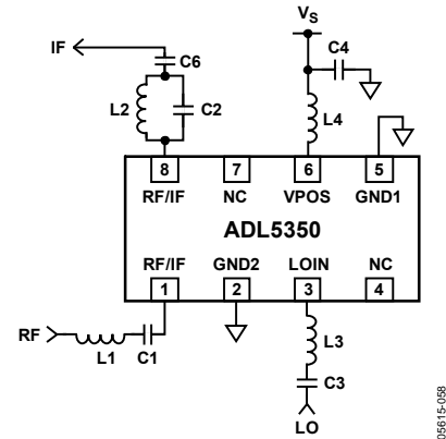
Figure 58. Reference Schematic
