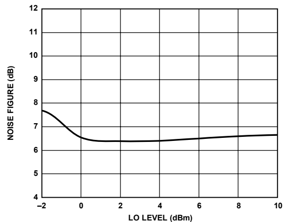
Figure 26. Noise Figure vs. LO Level
