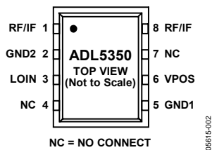
Figure 2. Pin Configuration
