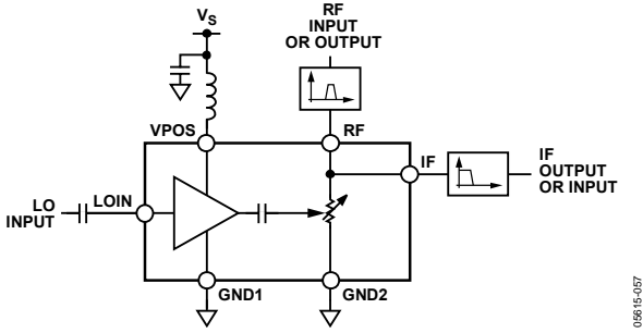
Figure 57. Simplified Schematic
