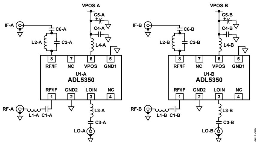
Figure 65. Evaluation Board
