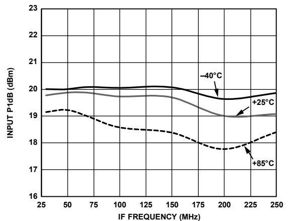
Figure 20. Input P1dB vs. IF Frequency
