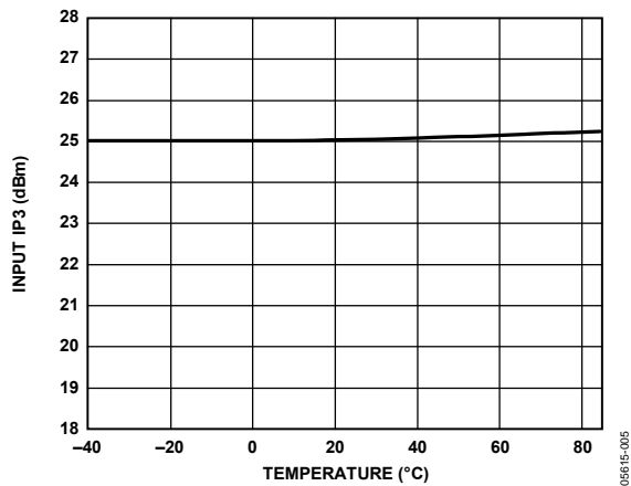
Figure 5. Input IP3 (IIP3) vs. Temperature
