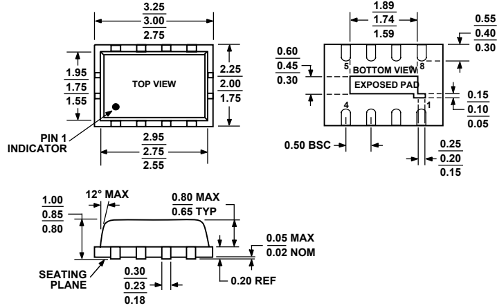
Figure 66. 8-Lead Lead Frame Chip Scale Package [LFCSP_VD] 2 mm × 3 mm Body, Very Thin, Dual Lead (CP-8-1) Dimensions shown in millimeters
