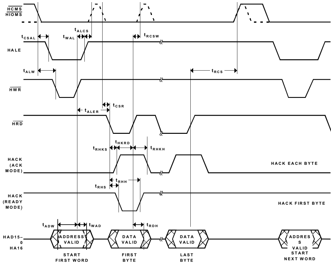
Figure 20. Host Port ACC Mode Read Cycle Timing
