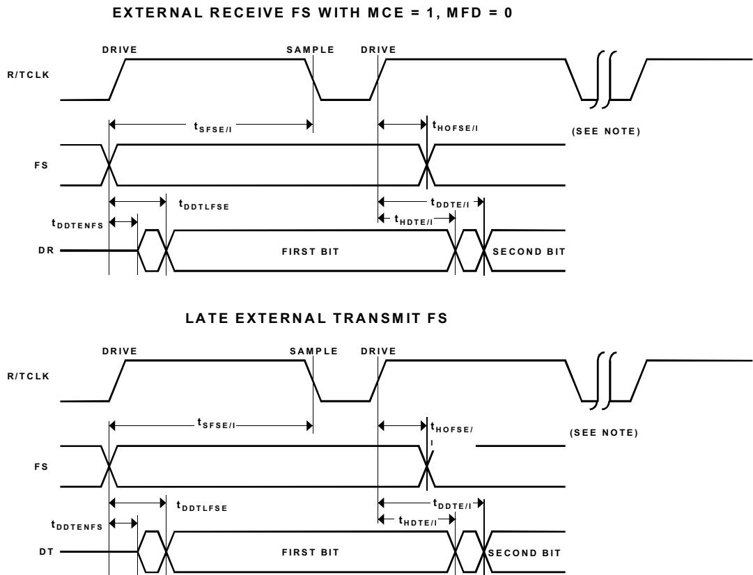
Figure 22. Serial Port (SPORT) Frame Synchron
