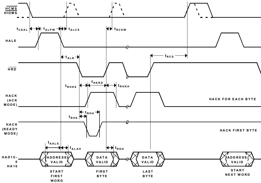
Figure 19. Host Port ALE Mode Read Cycle Timing
