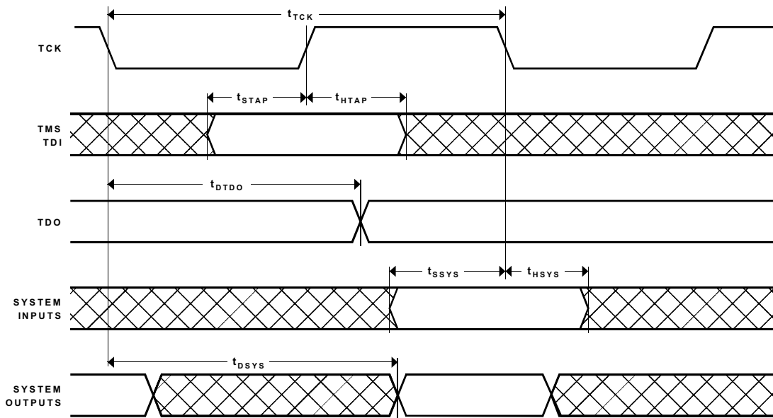
Figure 26. JTAG Port Timing
