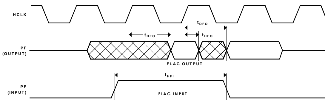
Figure 12. Programmable Flags Cycle Timing
