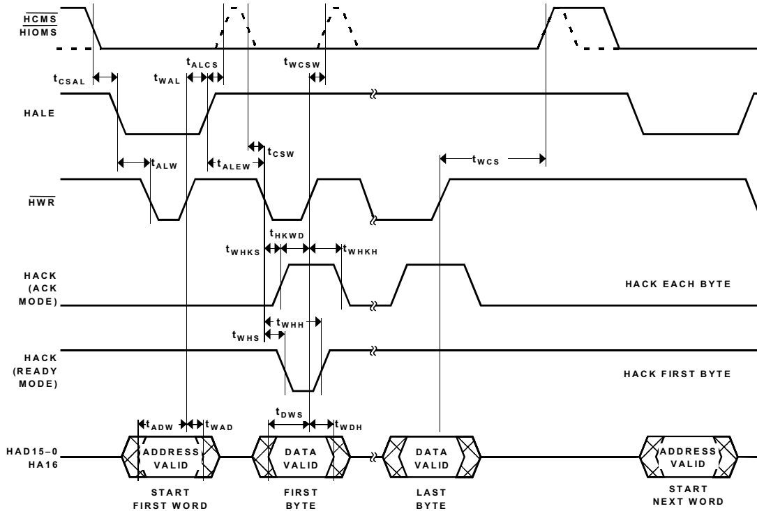
Figure 18. Host Port ACC Mode Write Cycle Timing
