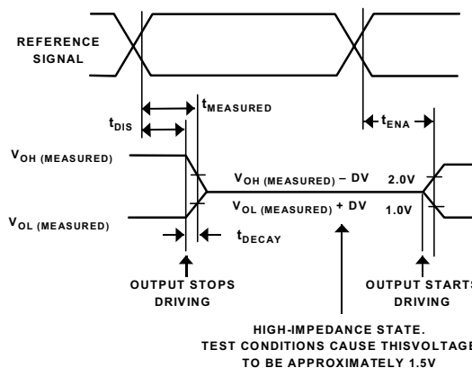
Figure 32. Output Enable/Disable
