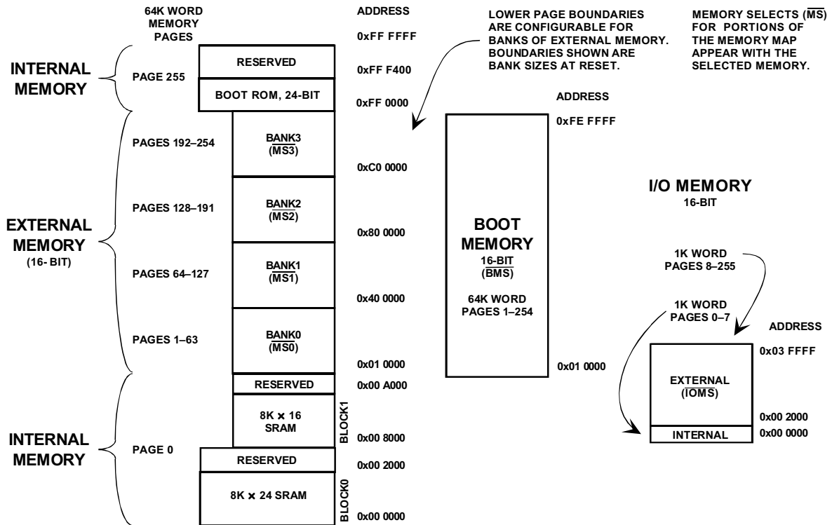
Figure 2. ADSP-2196 Memory Map
