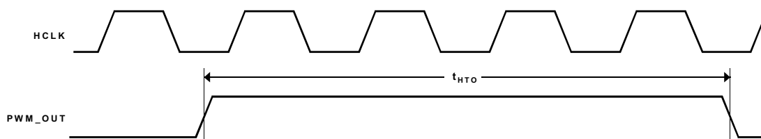
Figure 13. Timer PWM_OUT Cycle Timing
