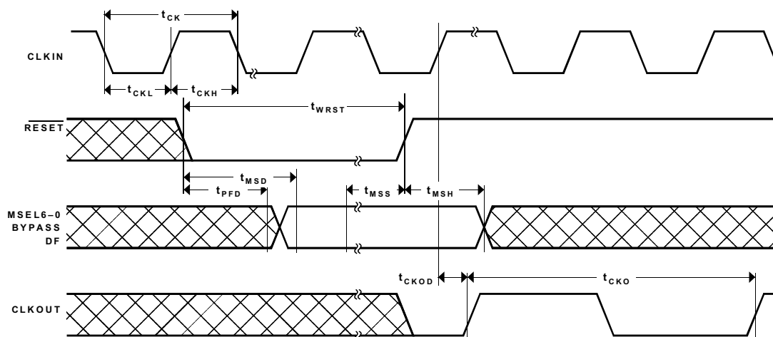
Figure 11. Clock In and Clock Out Cycle Timing
