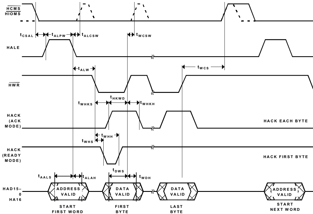
Figure 17. Host Port ALE Mode Write Cycle Timing
