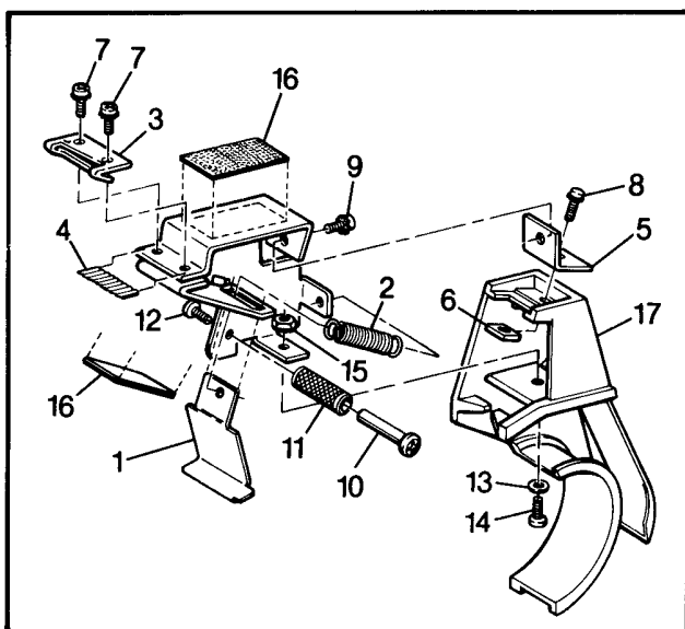
Figure 6 — Replacement Parts.
