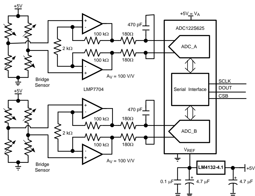
Figure 40. Interfacing the ADC122S625 to Bridge Sensors
