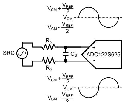
Figure 34. Differential Input
