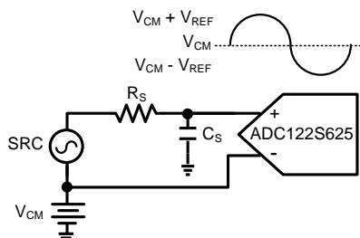
Figure 35. Single-Ended Input
