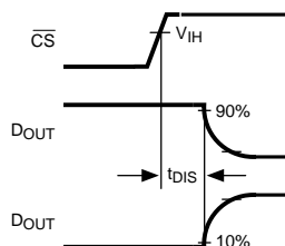
Figure 6. Voltage Waveform for t_{DIS}
