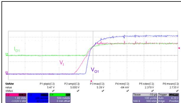
Figure 19. Startup transient (ST2S06B)
