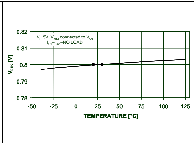
Figure 4. Feedback voltage 2 vs. temperature (ST2S06B)
