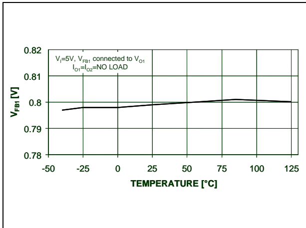
Figure 3. Feedback voltage 1 vs. temperature (ST2S06B)
