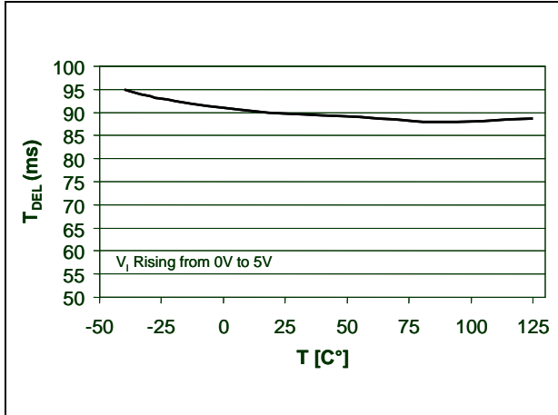
Figure 15. Delay time vs. temperature (ST2S06A33)
