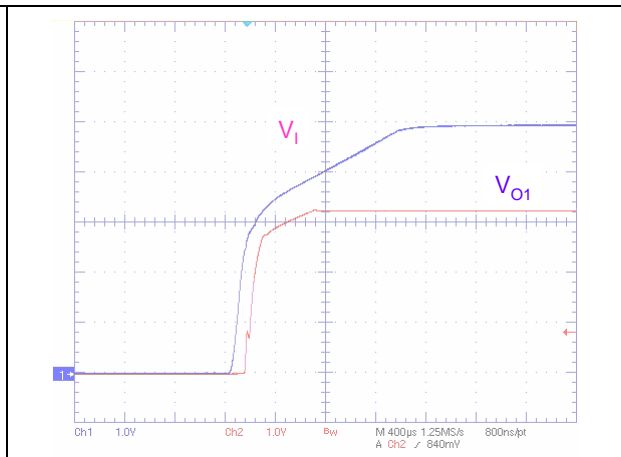
Figure 18. Startup transient (ST2S06A33)
