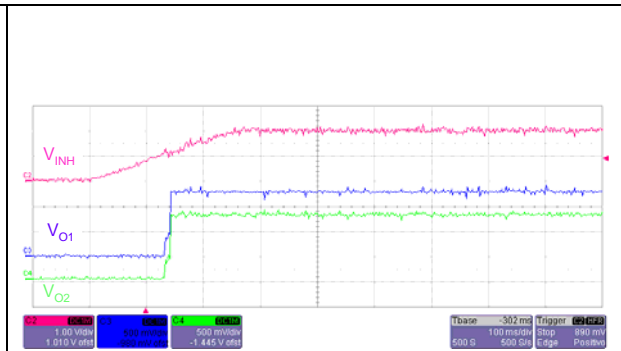
Figure 20. Inhibit transient (ST2S06B)
