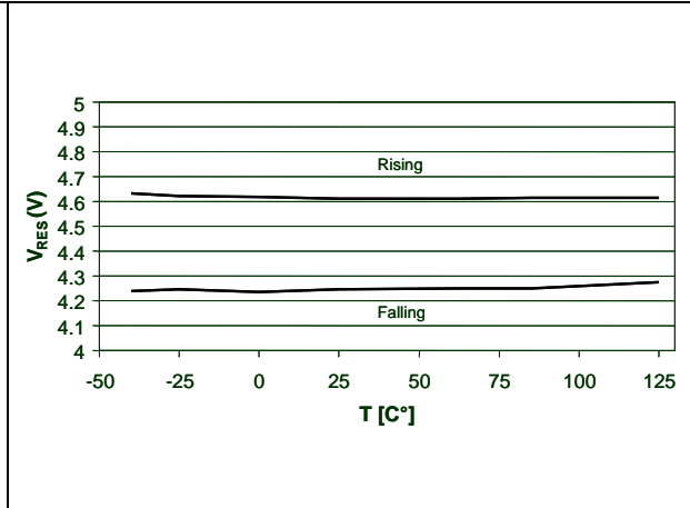
Figure 16. Reset in threshold vs. temperature (ST2S06A33)
