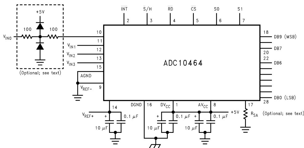
Figure 21. Typical Connection
