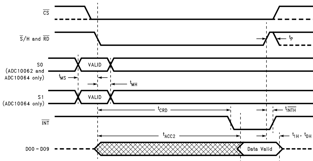
Figure 5. Mode 2 ( \overline{RD} Mode)
