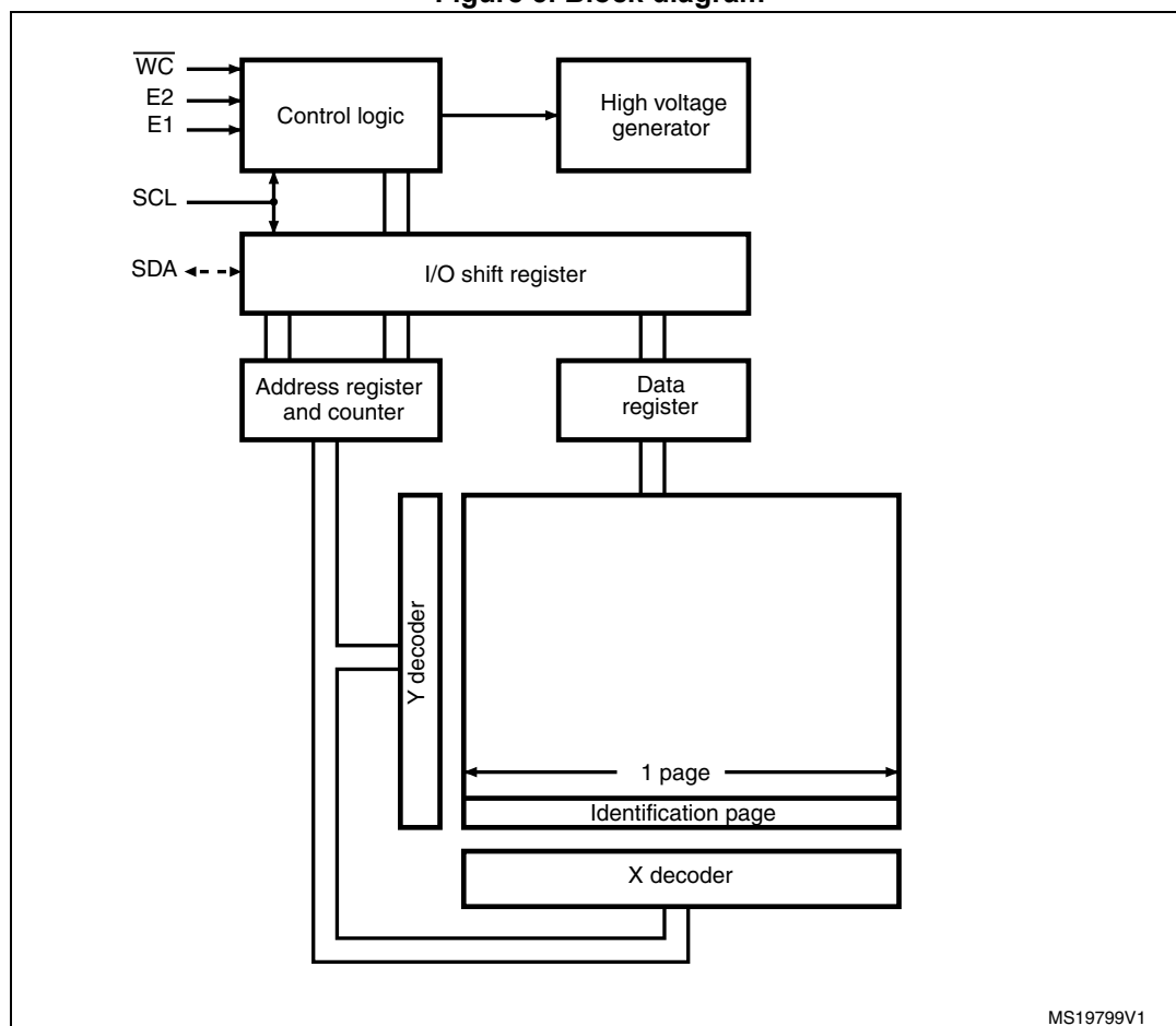
Figure 5. Block diagram
