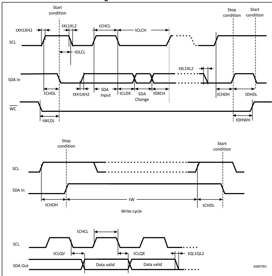
Figure 14. AC waveforms
