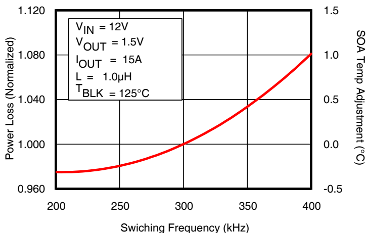
Fig. 6: Normalized Power Loss vs. Frequency
