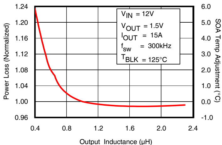
Fig. 7: Normalized Power Loss vs. Inductance
