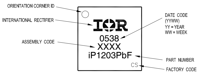
Fig. 27: Part Marking
