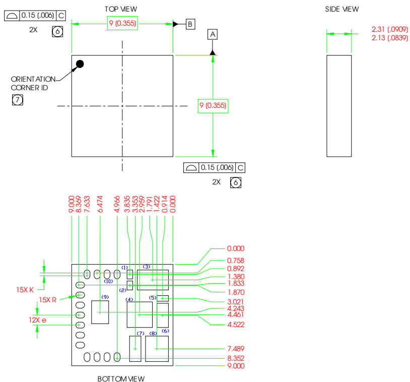
Fig. 25: Outline Drawing
