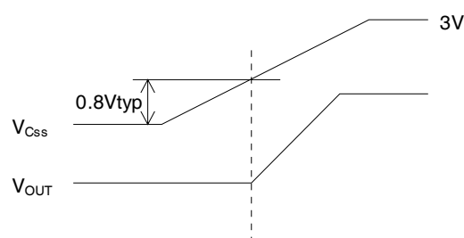
Fig. 13: Power Up Threshold
