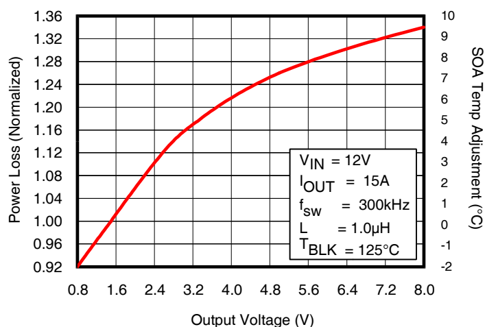
Fig. 5: Normalized Power Loss vs. V_{OUT}
