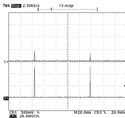
Ch1: Output voltage, 500mV/div Ch3: Output current, 10A/div
