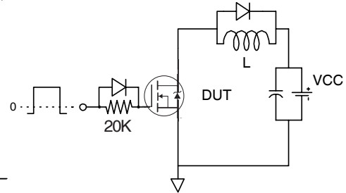
Fig 15. Gate Charge Test Circuit
