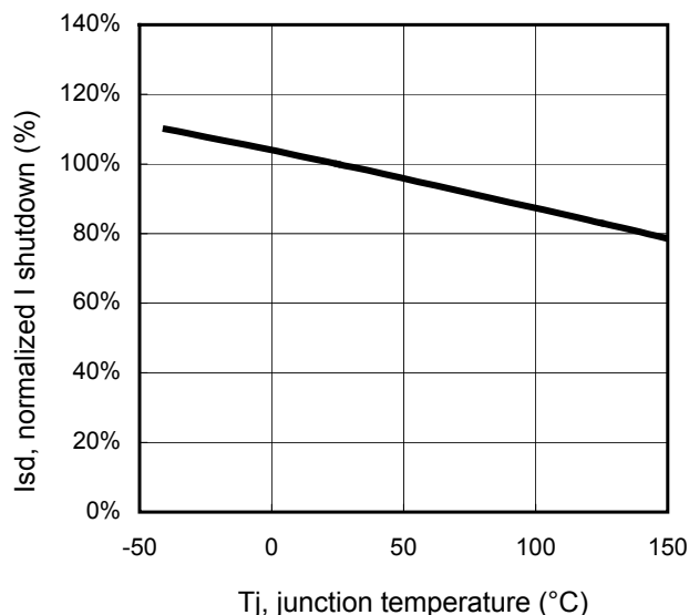
Figure 8 – Normalized I shutdown (%) Vs junction temperature (°C)
