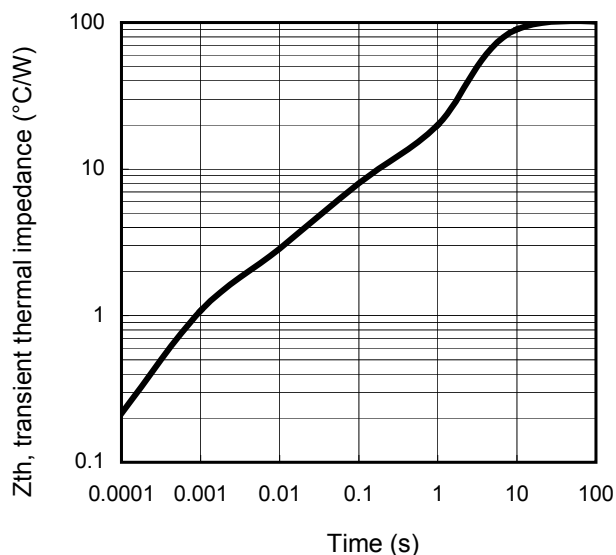
Figure 12 – Transient thermal impedance (°C/W) Vs time (s)
