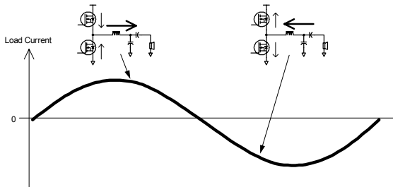
Direction in MOSFET Current and Load Current
