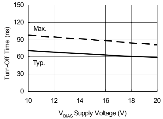
Figure 7B. Turn-Off Time vs. Supply Voltage
