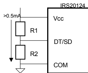
External Resistor
