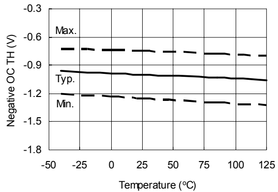
Figure 32. Negative OC Threshold(-) in V_S vs. Temperature
