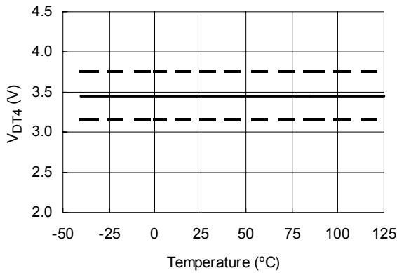
Figure 29. DT Mode Select Threshold (4) vs. Temperature
