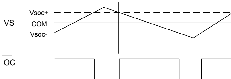
Figure 5. OC Waveform Definitions
