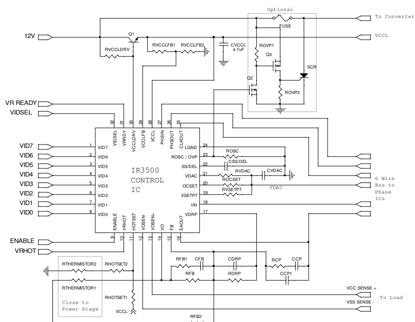
Figure 1 – Application Circuit
