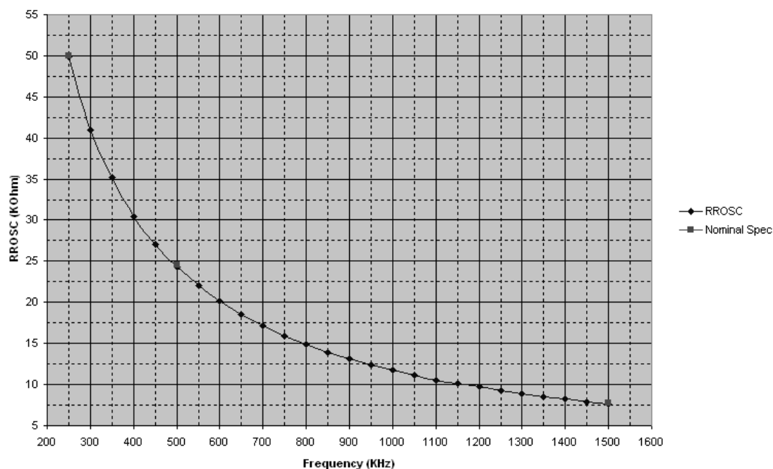
Figure 23 - Frequency variation with ROSC.
