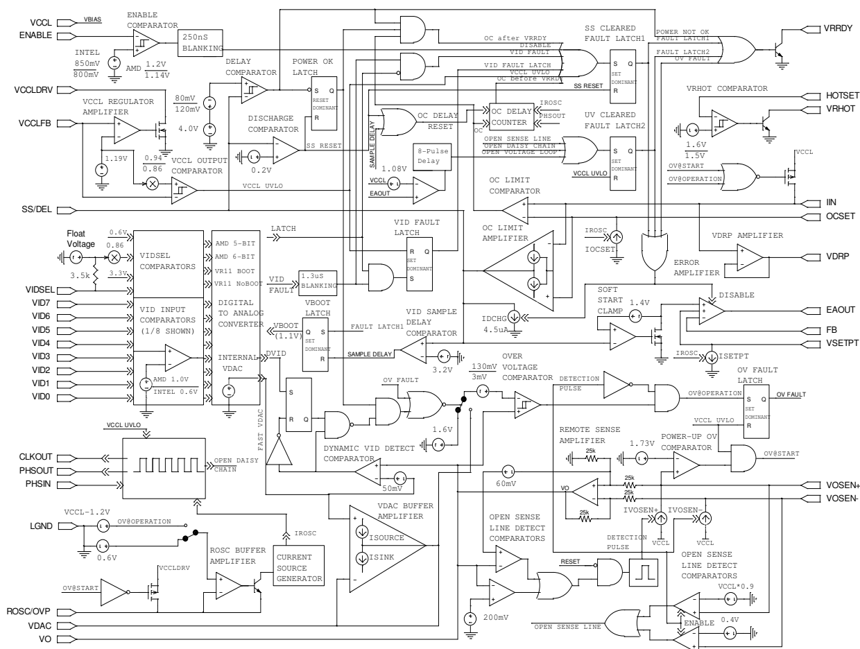
Figure 8 - Block Diagram
