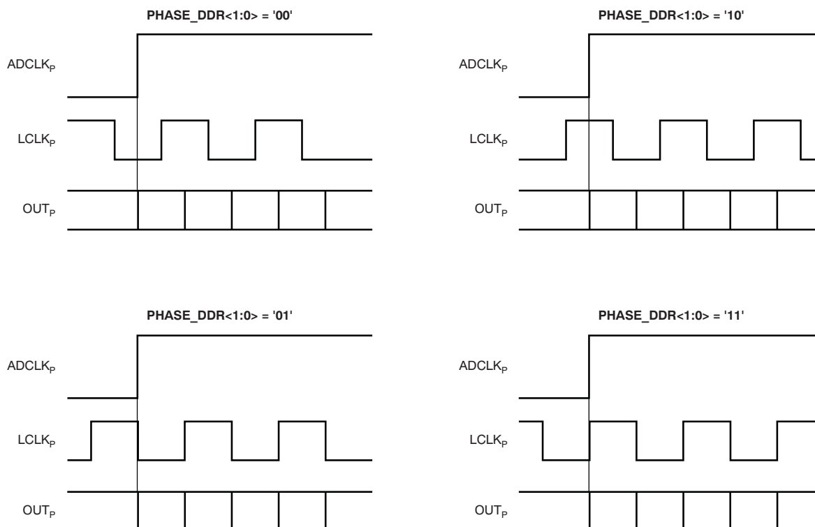
Figure 2. Phase Programmability Modes for LCLK
