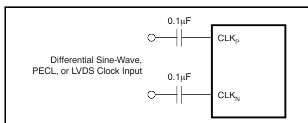
Figure 37. Differential Clock Driving Circuit ( \text{DIFF\_CLK} = 1 )
