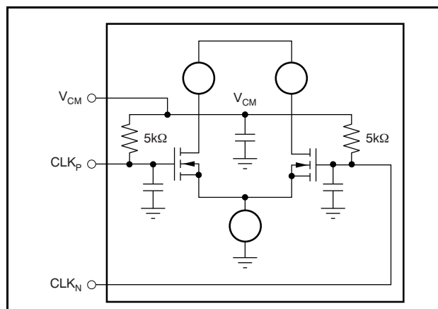
Figure 36. Internal Clock Buffer
