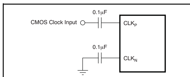
Figure 38. Single-Ended Clock Driving Circuit When \text{DIFF\_CLK} = 1
