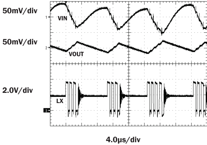
PSAVE @ 50mA Load with C_{OUT} = 22\mu F
