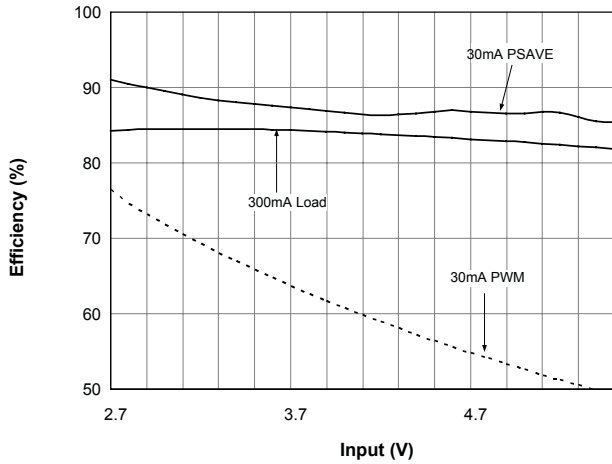
Efficiency vs. Line @ V_{OUT} = 1.8V
