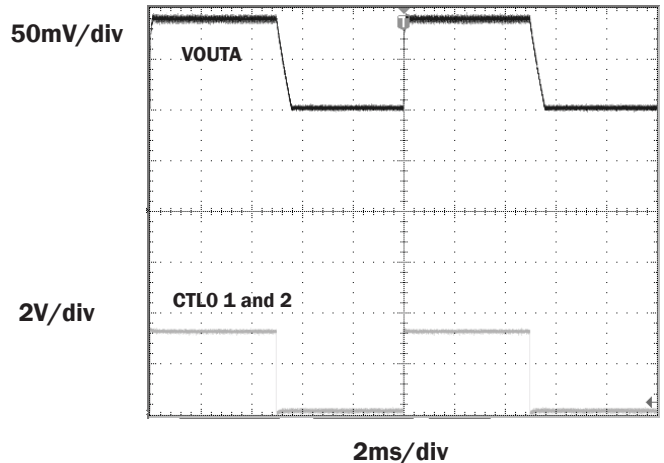
Output Transient in PSAVE
