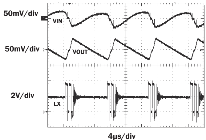
PSAVE @ 30mA Load
