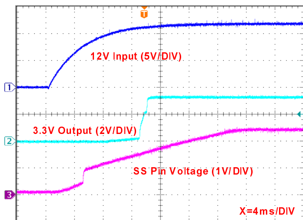
Figure 13(c). 12VIN start-up transient at 2A load.
