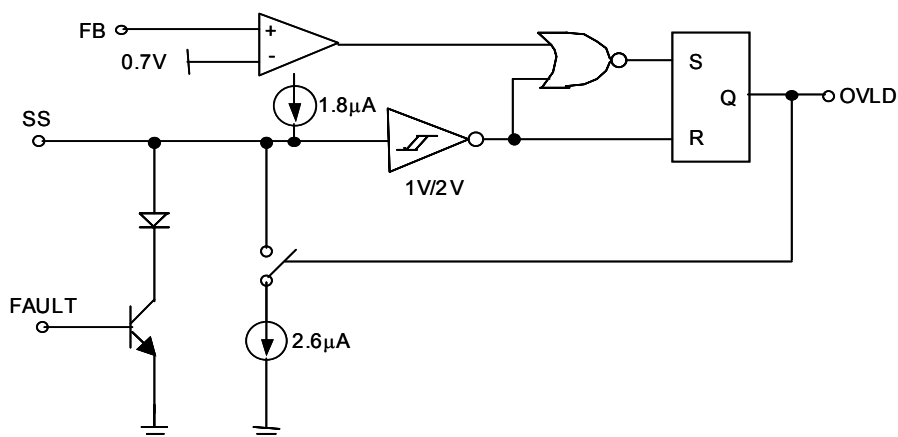
Figure 3. Details of the Soft-Start and Overload Hiccup Control Circuit
