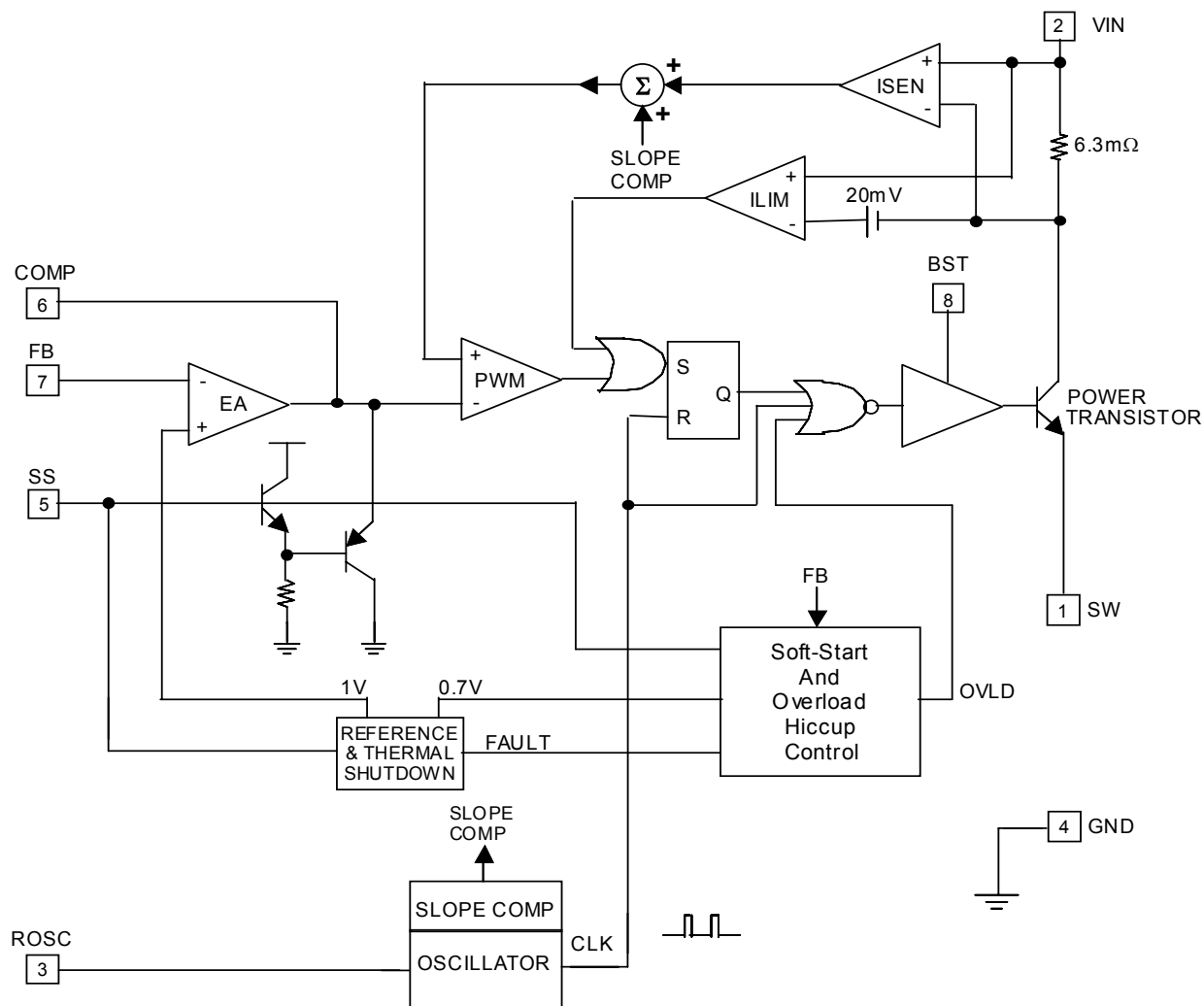
Figure 2. SC4524 Functional Diagram
