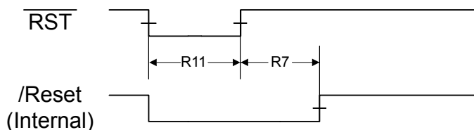
Figure 24-4. External Reset Timing ( \overline{RST} )
