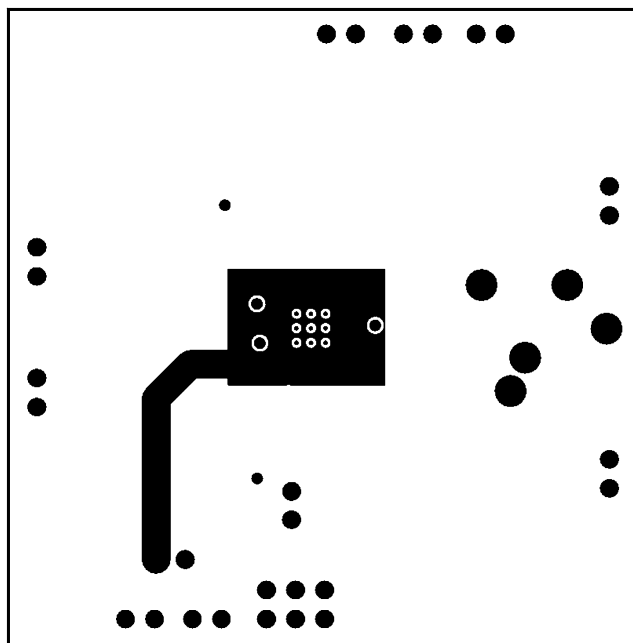
Figure 39. Recommended SP PCB Layout: Mid Layer
