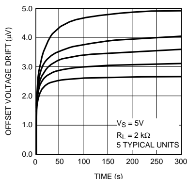
Figure 44. Start-Up Input Offset Voltage Drift
