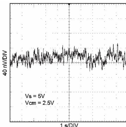
Figure 43. 0.1 Hz to 10 Hz Input Voltage Noise
