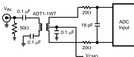
Figure 21. Low Input Frequency Transformer Drive Circuit
