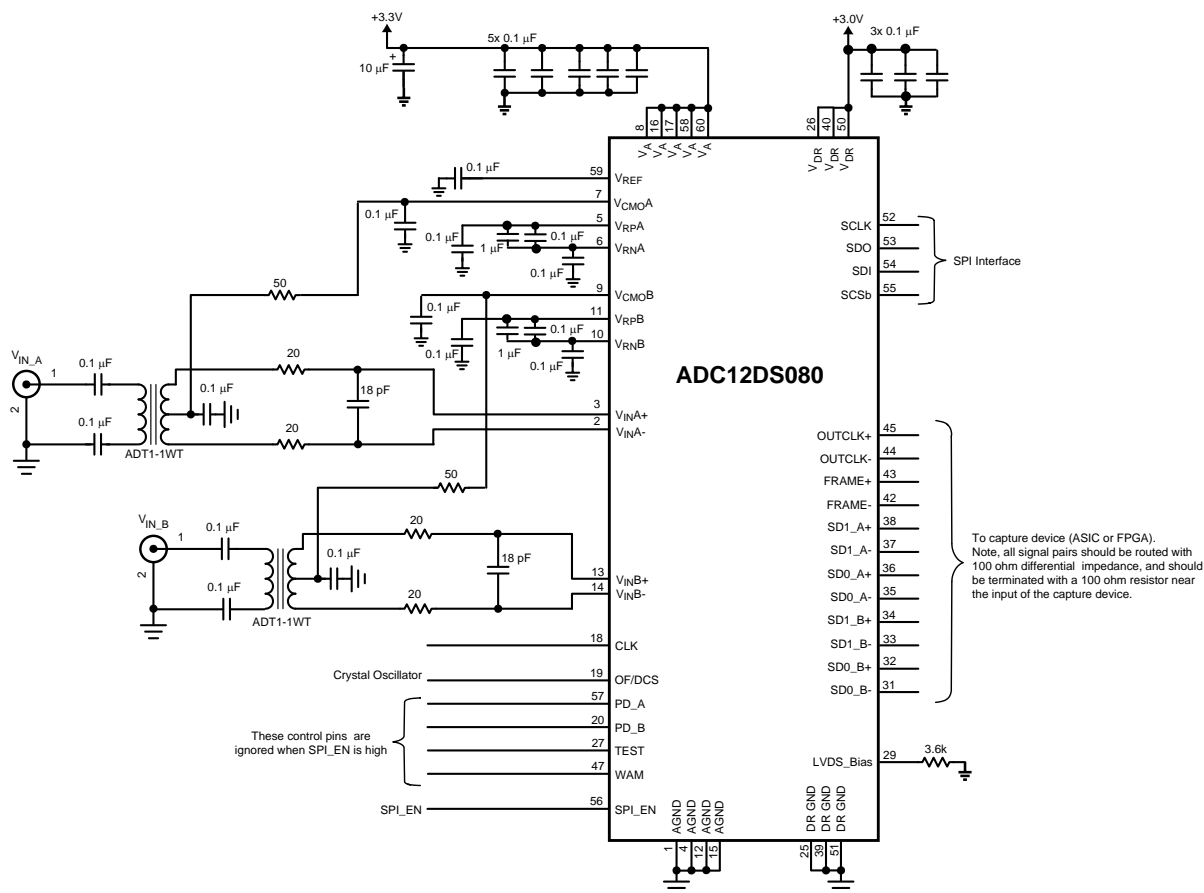
Figure 23. Application Circuit
