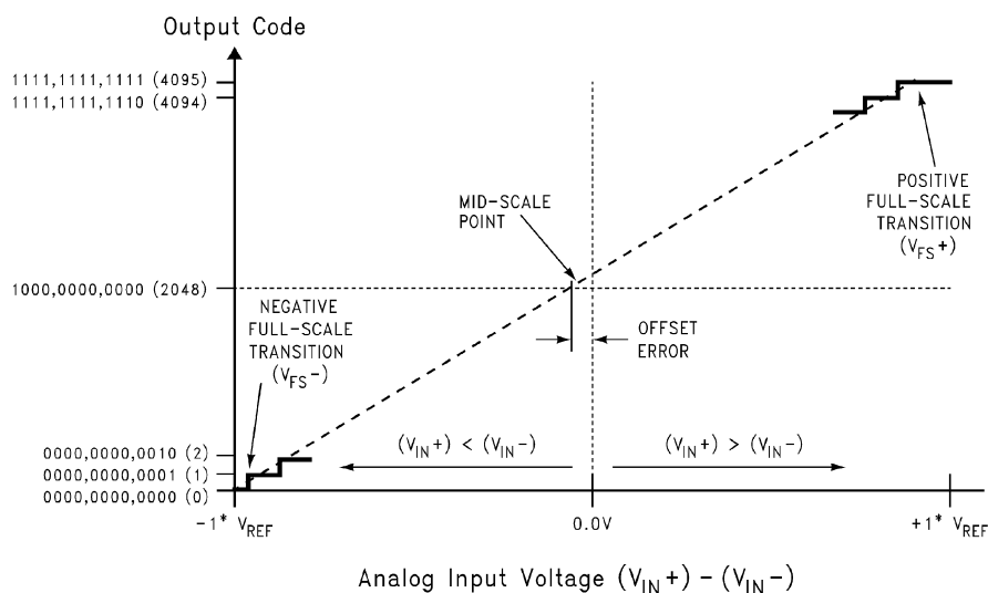
Figure 6. Transfer Characteristic
