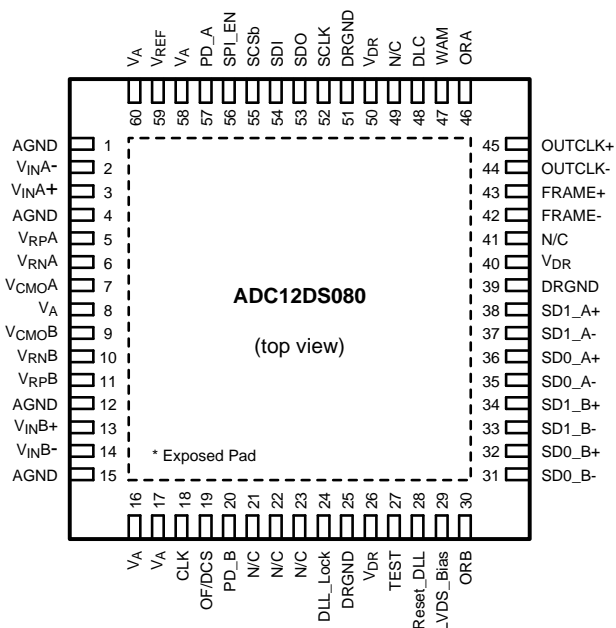
Figure 1. WQFN Package See Package Number NKA0060A
