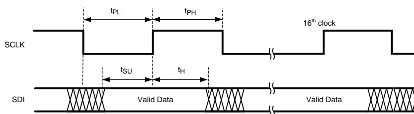
Figure 26. Write Timing
