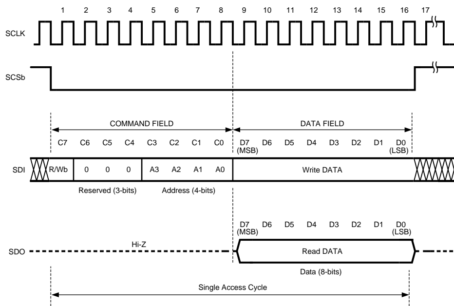
Figure 24. Serial Interface Protocol
