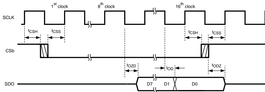
Figure 25. Read Timing
