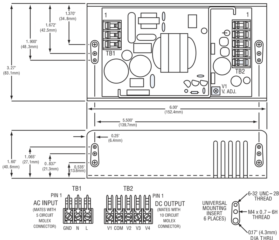
Figure-1 - Mechanical Drawing
