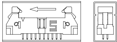
FIG 5 THROUGH HOLE (SEE NOTE 6)
