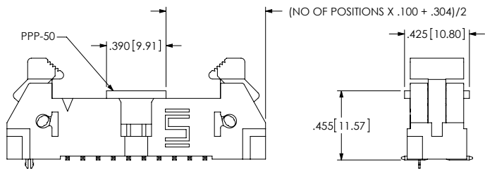
FIG 6 -P: PICK & PLACE PAD
