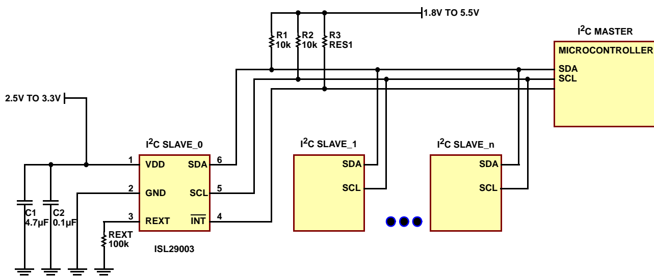
FIGURE 7. ISL29003 TYPICAL CIRCUIT
