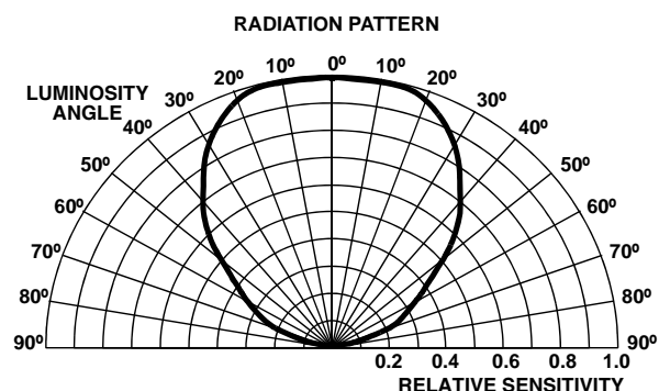
FIGURE 9. RADIATION PATTERN
