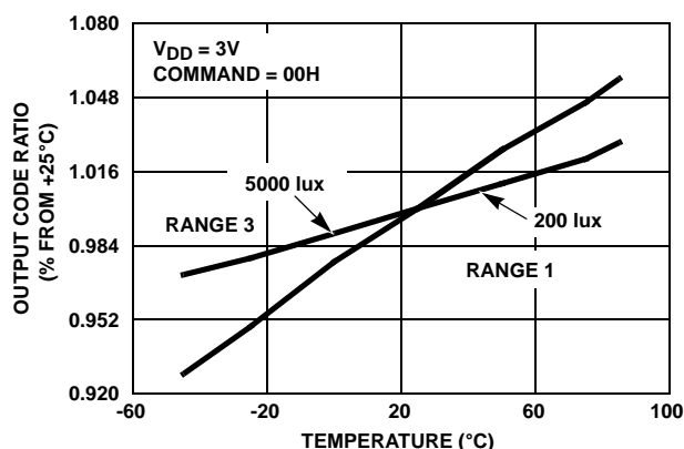
FIGURE 16. OUTPUT CODE vs TEMPERATURE
