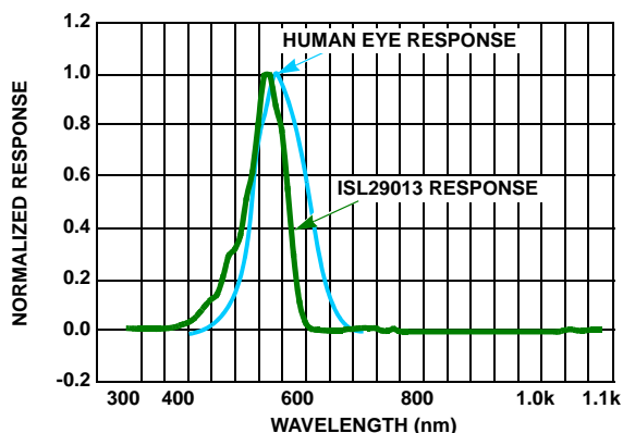
FIGURE 6. SPECTRAL RESPONSE
