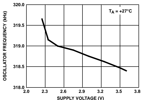
FIGURE 12. OSCILLATOR FREQUENCY vs SUPPLY VOLTAGE
