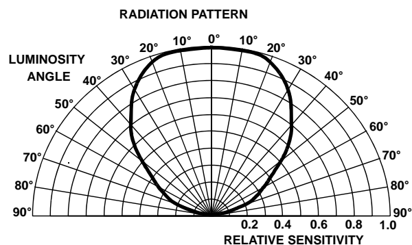
FIGURE 7. RADIATION PATTERN
