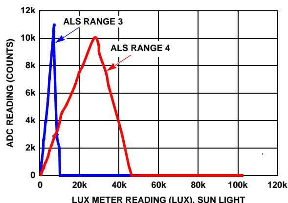
FIGURE 17. SATURATION CHARACTERISTICS
