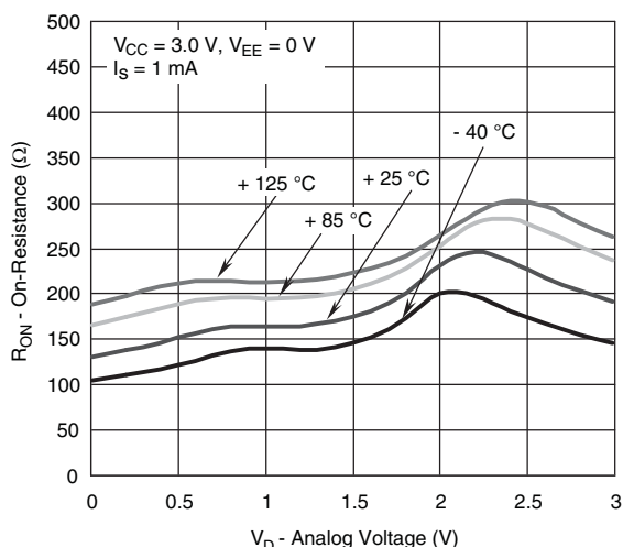
On-Resistance vs. Analog Voltage and Temperature at V_{CC} = +3 V, V_{EE} = 0 V
