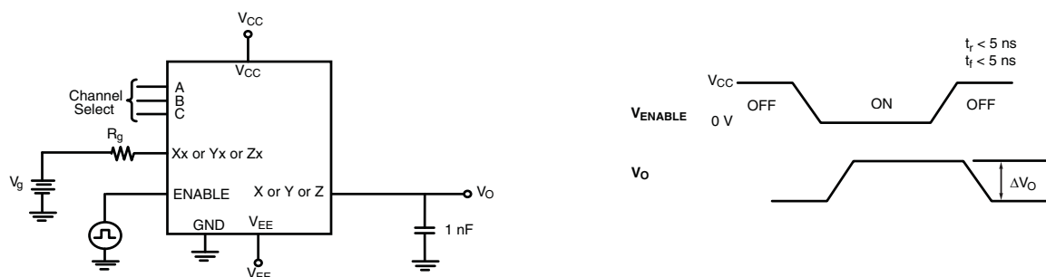
Figure 4. Charge Injection
