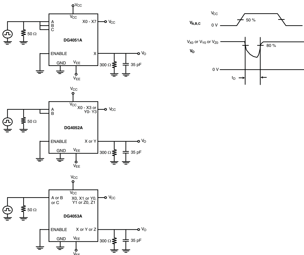
Figure 3. Break-Before-Make
