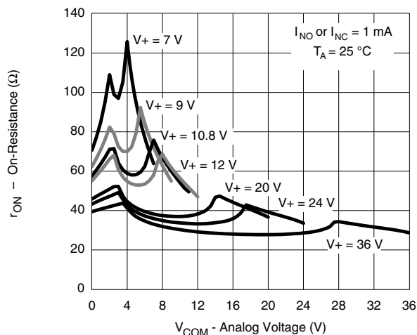
On Resistance vs. V_{COM} and Single Supply Voltage
