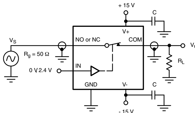
Figure 4. Insertion Loss
