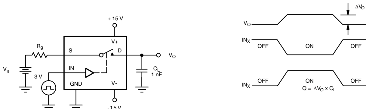
Figure 3. Charge Injection
