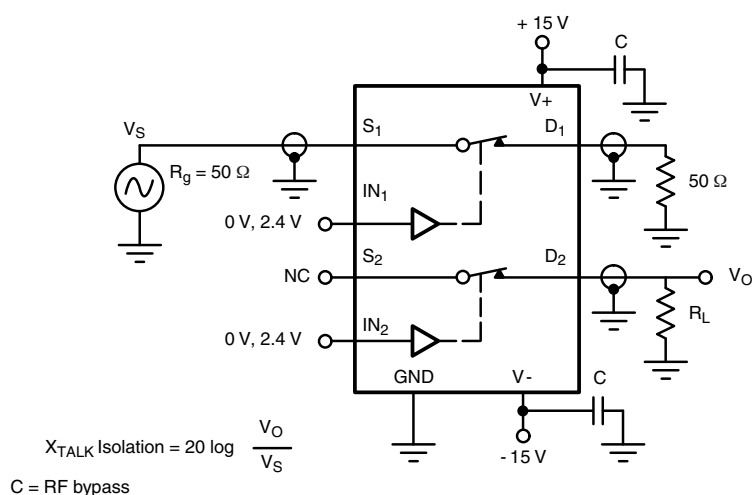
Figure 4. Crosstalk
