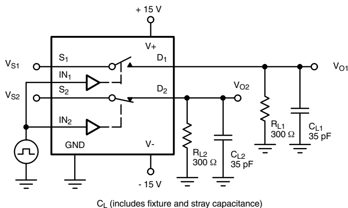
Figure 2. Break-Before-Make (DG456)
