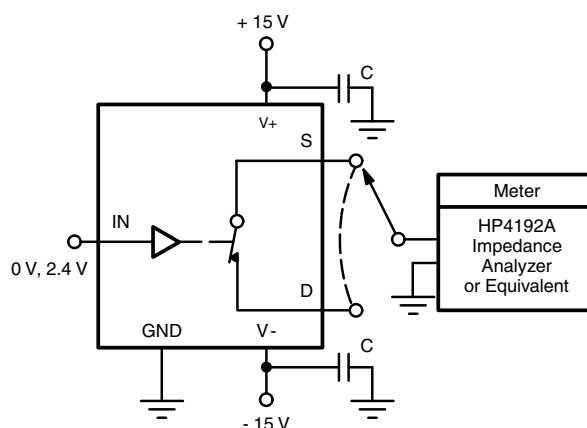
Figure 6. Source/Drain Capacitances
