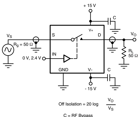
Figure 5. Off-Isolation
