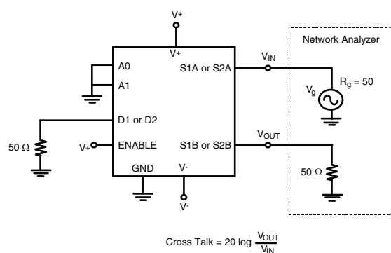
Fig. 6 - Crosstalk
