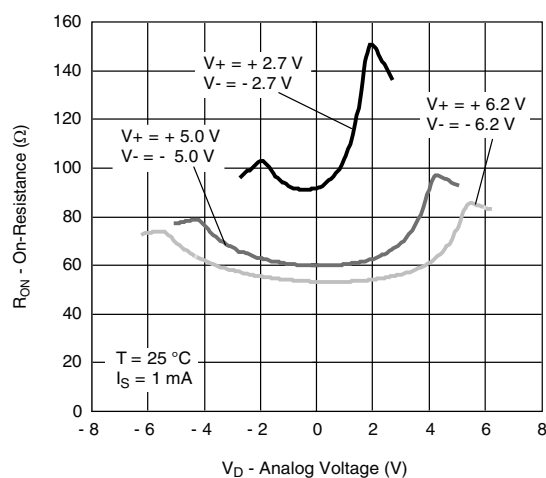
On-Resistance vs. V_D (Dual Supply Voltage)
