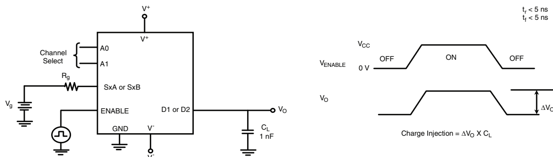
Fig. 4 - Charge Injection
