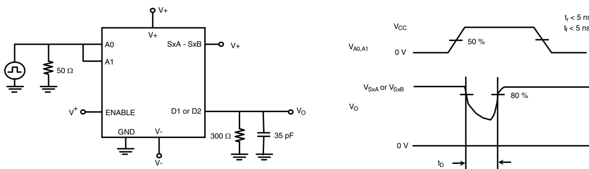
Fig. 3 - Break-Before-Make
