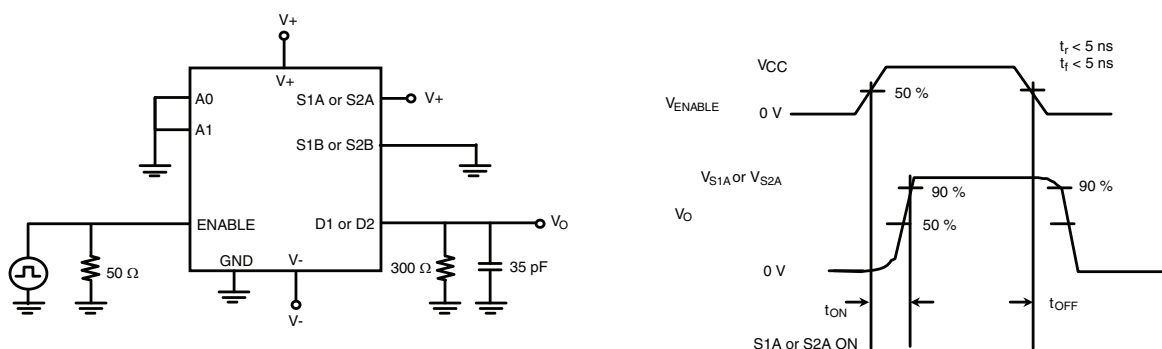
Fig. 2 - Enable Switching Time
