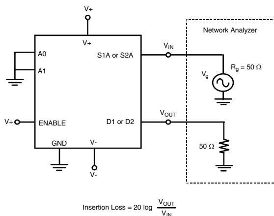
Fig. 5 - Insertion Loss
