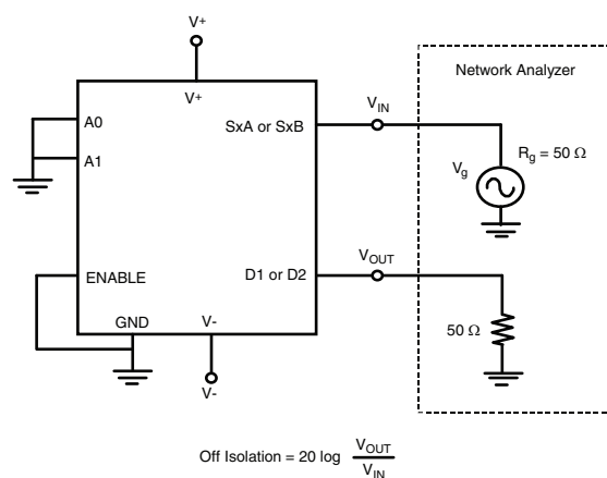
Fig. 7 - Off-Isolation
