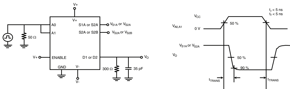
Fig. 1 - Transition Time
