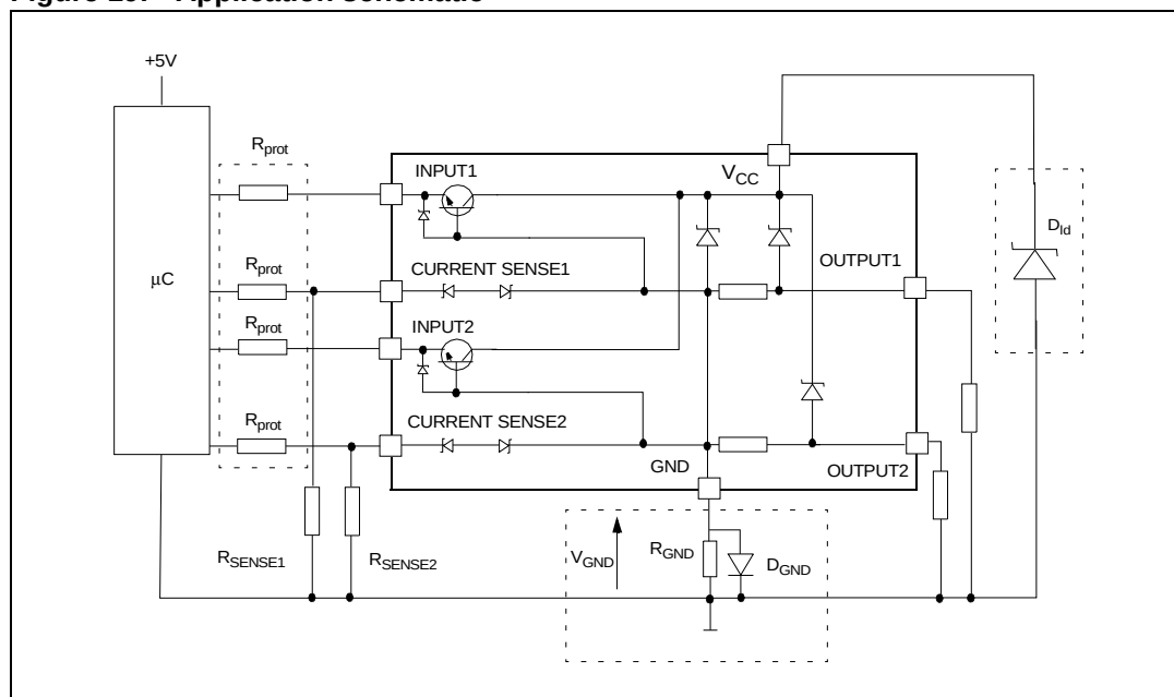
Figure 19. Application schematic
